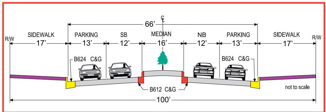
Lyndale Avenue Roadway Typical Section 66 Ft. Curb to Curb – West Minnehaha Parkway to 56th Street West
